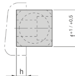
Passung / Seat
