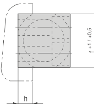
Passung / Seat
